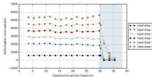
Figure 5. Deformation along the ground anchor at different steps of the load test. The bonded length is indicated by the shaded zone.
